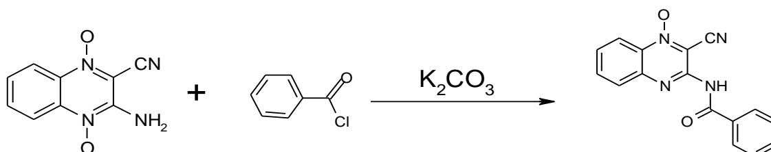
Scheme 2: The synthesis of 2-benzamide-3-cyanoquinoxaline-4-oxide, (I)
