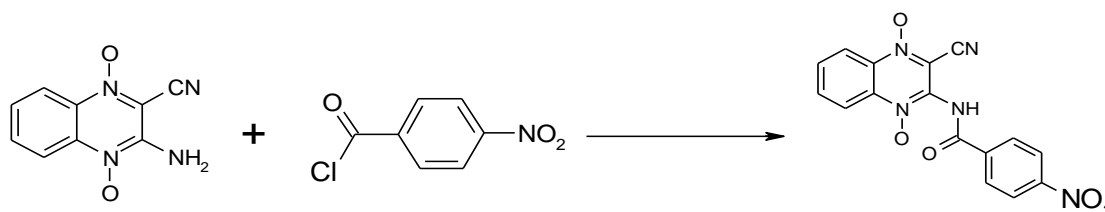
Scheme 3: The synthesis of N -(3-cyano-1,4-dioxy-quinoxaline-2-yl)-4-nitro-benzamide, (II).
