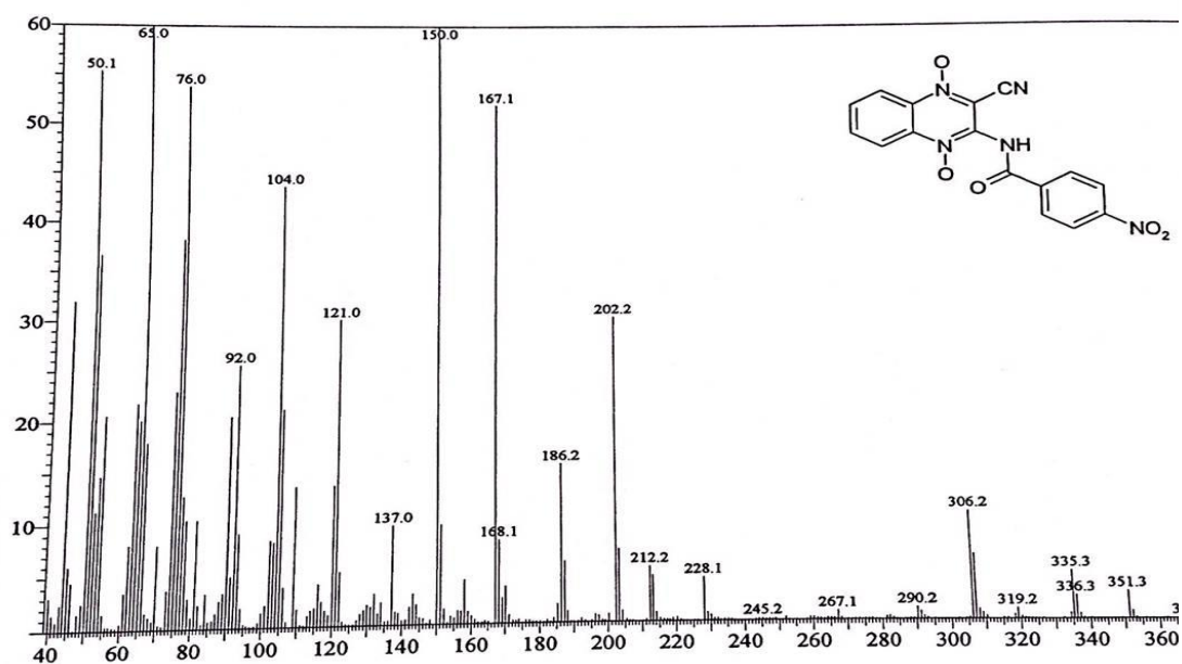
Figure 2: The ESI-MS spectrum of compound II, C 16 H 9 N 5 O 5
