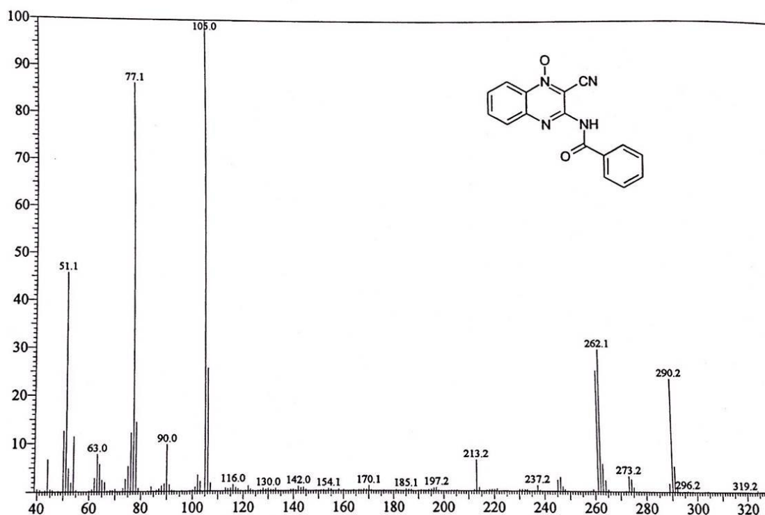
Figure 1: The ESI-MS spectrum of compound I, C 16 H 10 N 4 O 2
